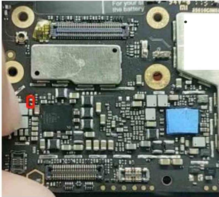
Drop diode position diagram
